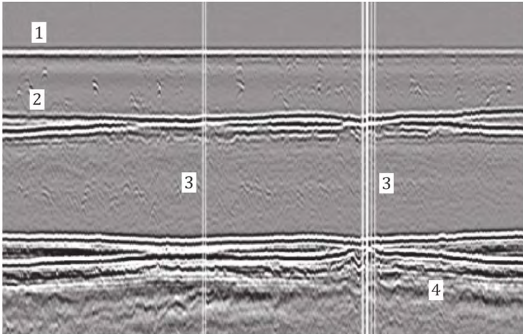
Key 1 lateral wave 3 missing scan lines 2 back-wall reflection 4 mode-converted signal
