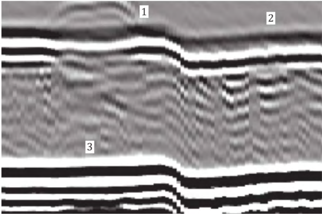
Key 1 indication 3 mode-converted signal 2 back-wall reflection Lateral wave is not present in the time window.
