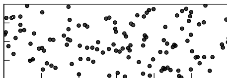
Figure A.8 — 8 surface percent, 122 pores, d = 1 mm
