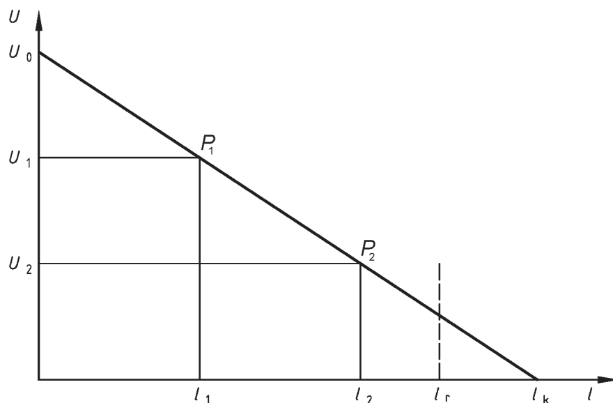
Figure 2 — Load characteristics of the current generator
