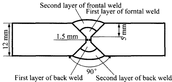
图 1 焊接坡口尺寸和焊接顺序示意图 Fig. 1 Schematic diagram of welding groove dimensions and welding sequence
