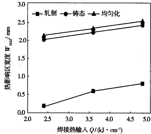
图 4 不同焊接热输入下各母材焊接接头 HAZ 宽度 Fig. 4 Width of HAZ in different base metal welding joint using different heat input
