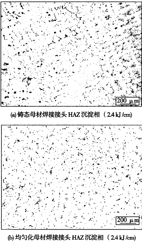
图 3 铸态与均匀化母材焊接 HAZ 微观组织差异 Fig. 3 Microstructure difference in HAZ between as-cast and homogenized base metal
