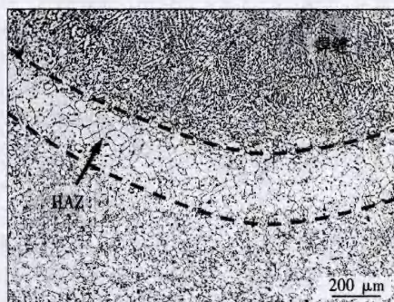
(a) 轧制母材焊接接头横截面金相 (2.4 kJ/cm)
