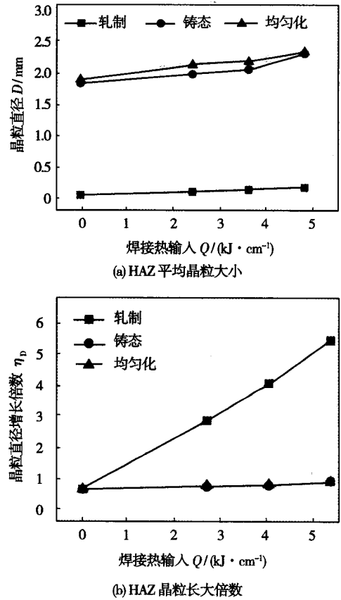
图 5 不同焊接热输入下各母材焊接接头晶粒大小及晶粒长大倍数 Fig. 5 Grain size and multiple grain growth of different base metal welding joint using different heat input
