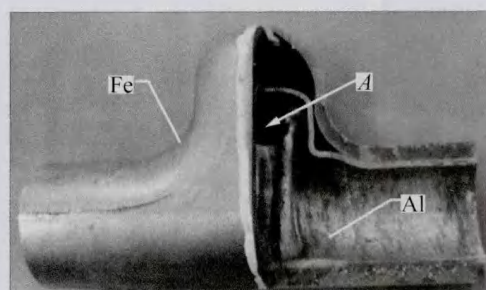
Fig. 11 View of failure after hydroforming process
