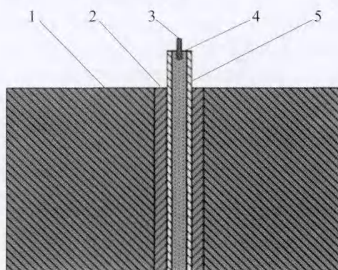
Fig. 1 Schematic diagram of arrangement: 1—Mould; 2—Ferrite tube; 3—Detonator; 4—Explosive; 5—Aluminium tube
