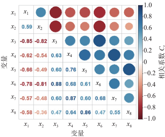
图 10 变量间相关性检验 Fig. 10 Correlation test between variables
