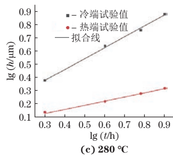
Fig. 7 Relationship between thickness of intermetallic compound layer and reflow time period at hot and cold ends of joint at different reflow temperatures
