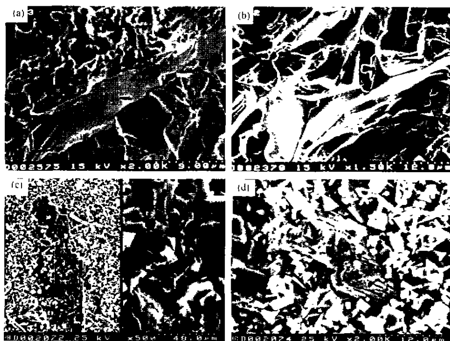
Fig 2 Morphology of NiCrSiB coating after cavitation erosion
