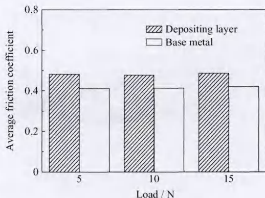
图8 不同载荷下母材与熔敷层平均摩擦因数 Fig. 8 Average friction coefficient of base metal and depositing layer under different loads
