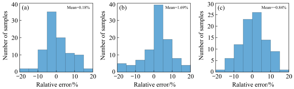
Fig. 20 Relative error between predicted results and experimental data of FS for Al/Cu composite with 30% Al (a), 42% Al (b), and 51% Al (c)
