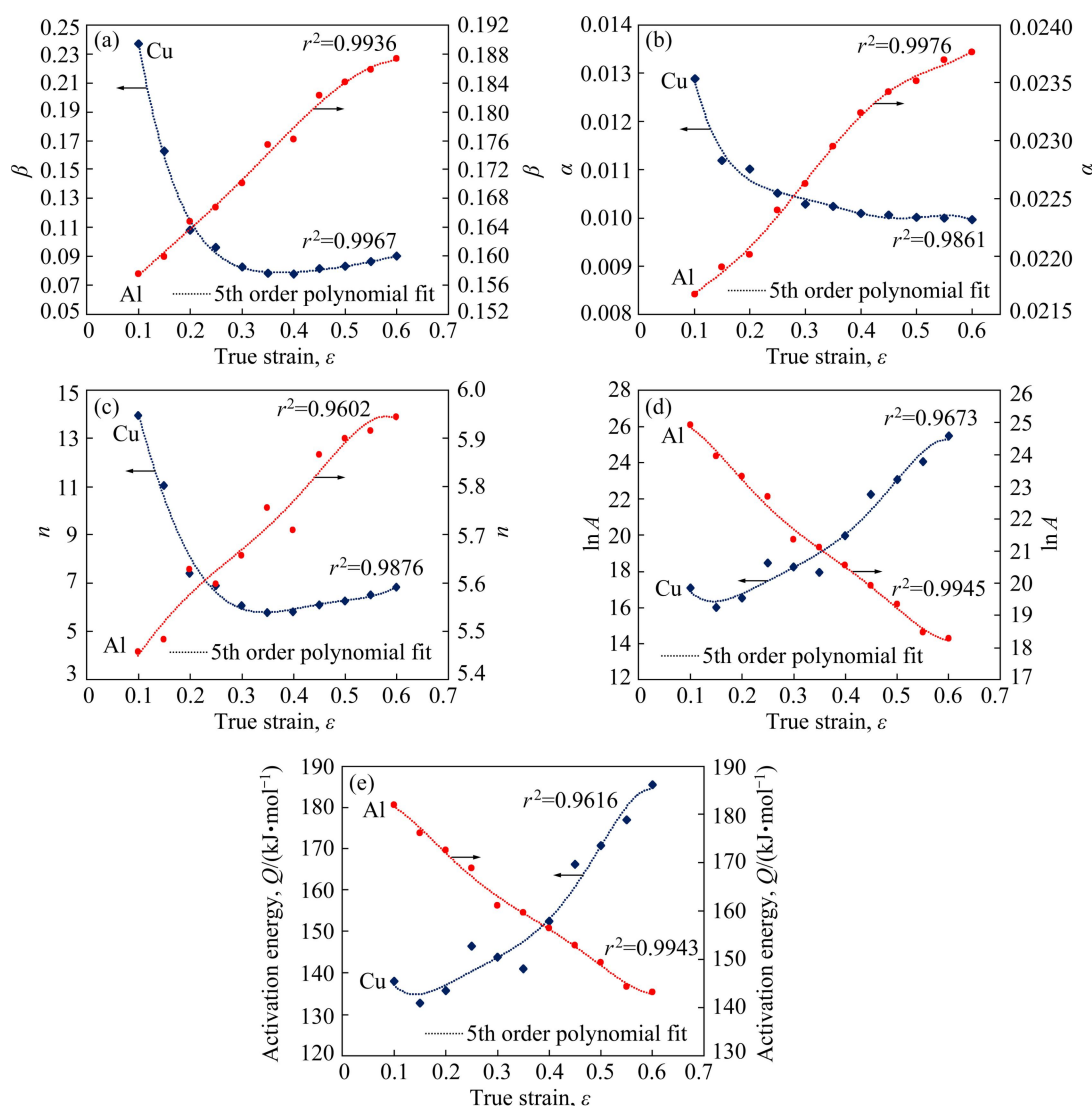
Fig. 15 Relationship between Q , n , \beta , \ln A and \alpha and true strain ( \varepsilon ) for AA7022 alloy and copper
