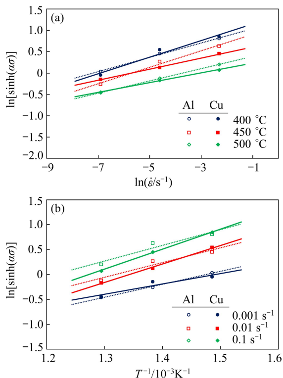
Fig. 12 Relationship plots between \ln \dot{\epsilon} and [\sinh(\alpha\sigma)] (a) and [\sinh(\alpha\sigma)] and (1/T) (b)
