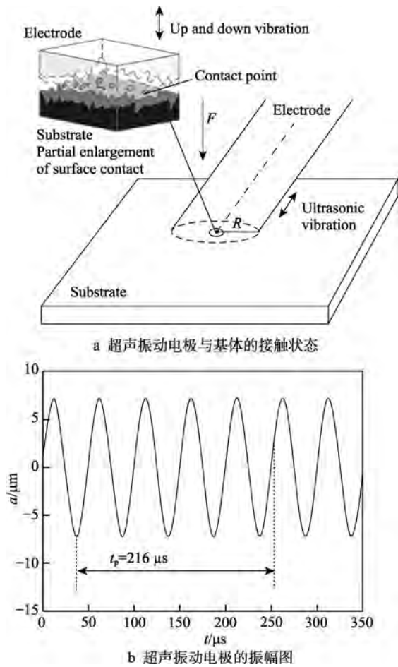
图 9 超声振动电极与基体的接触状态和电极振幅图 Fig.9 Contact state between ultrasonic vibrating electrode and substrate and amplitude diagram of electrode: a) contact state between ultrasonic vibrating electrode and substrate; b) amplitude diagram of ultrasonic vibrating electrode
