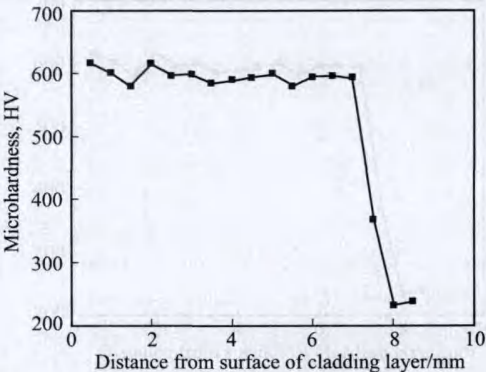
图 7 涂层沿厚度方向的显微硬度分布 Fig.7 Microhardness(HV) of cladding layer testing along thickness direction
