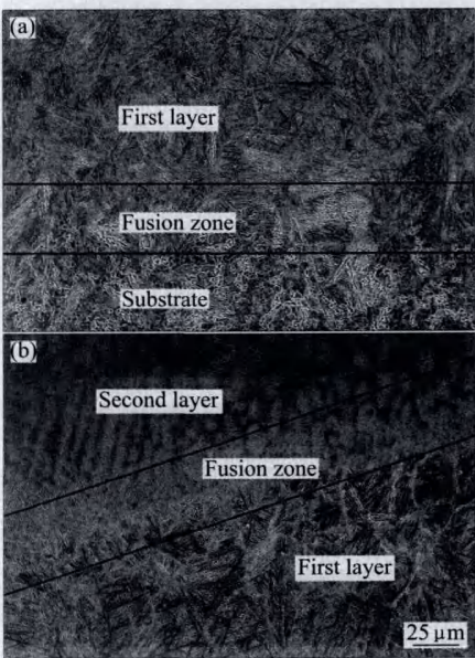
图 6 复合涂层熔合区的 SEM 像 Fig.6 SEM images of fusion zones of composite coatings: (a) Fusion zone between first layer and substrate; (b) Fusion zone between second layer and first layer
