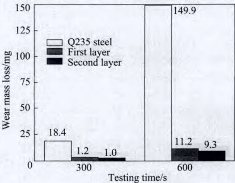
图 8 埋弧堆焊涂层和 Q235 钢磨损质量损失 Fig.8 Wear mass loss as function of time for composite coating as well as Q235 steel
