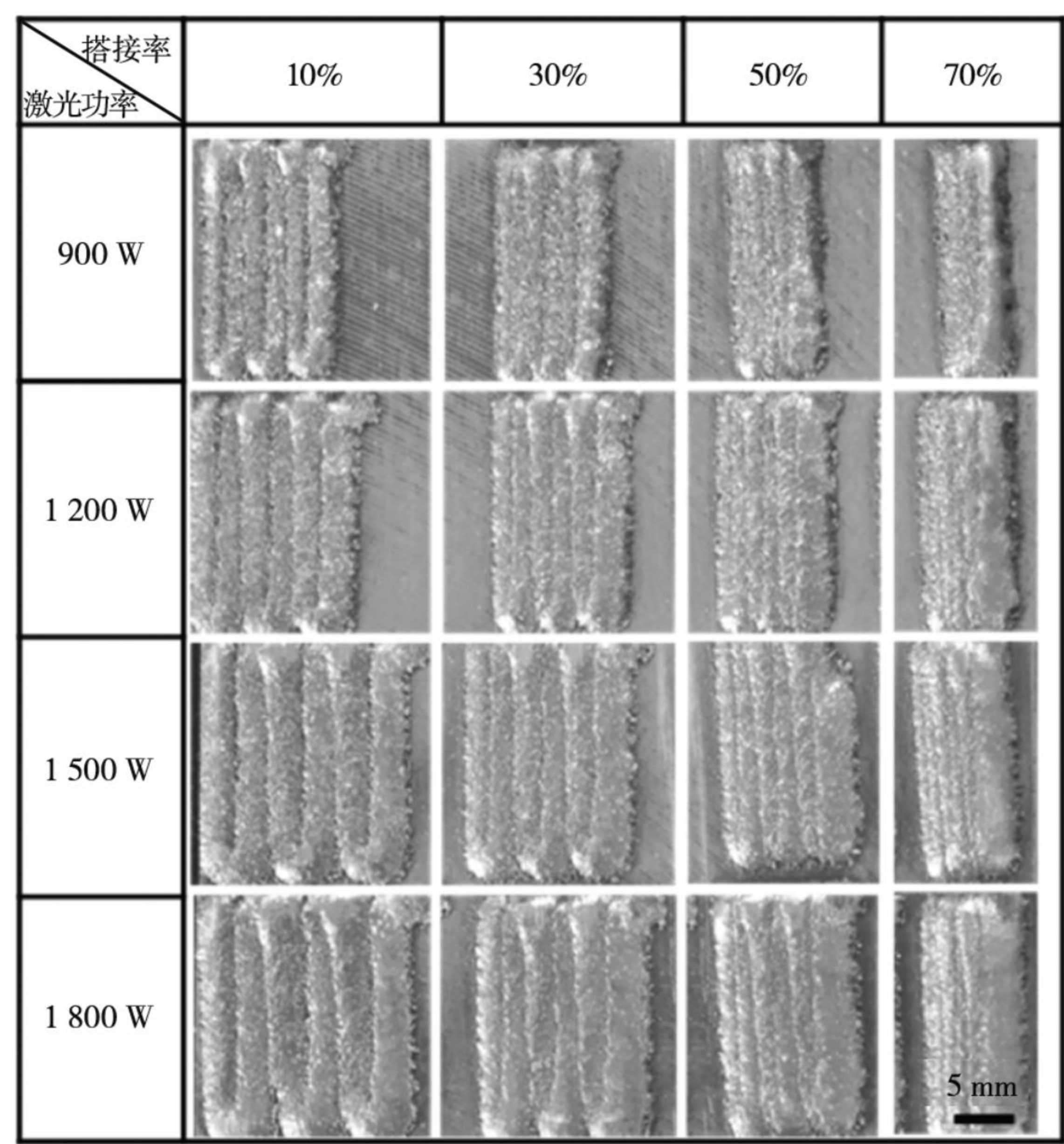
图6 不同搭接率与激光功率组合下LDED单层多道沉积表面形貌 Fig. 6 Surface morphologies of single-layer multi-pass LDED deposits under different lap joint rate and laser power combinations
