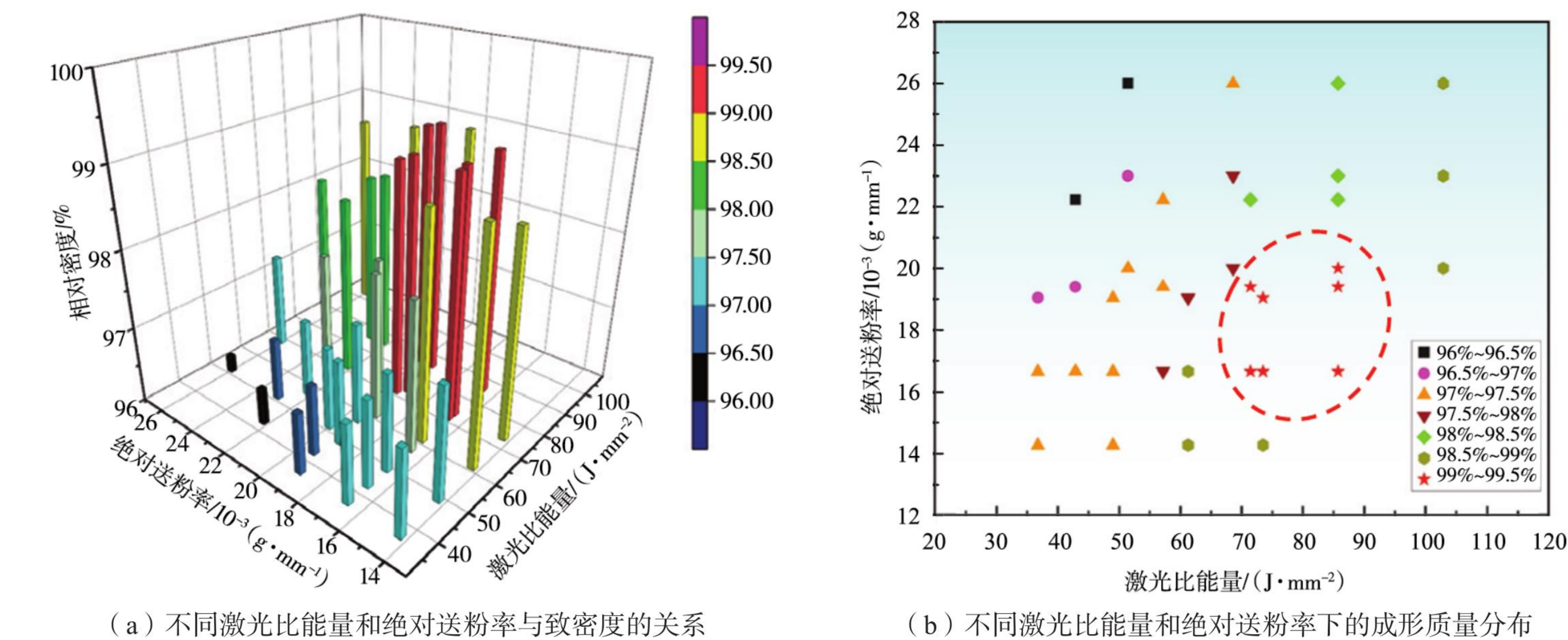
图8 不同工艺参数与合金致密度的关系 Fig. 8 Relationships between different process parameters and alloy compactnesses
