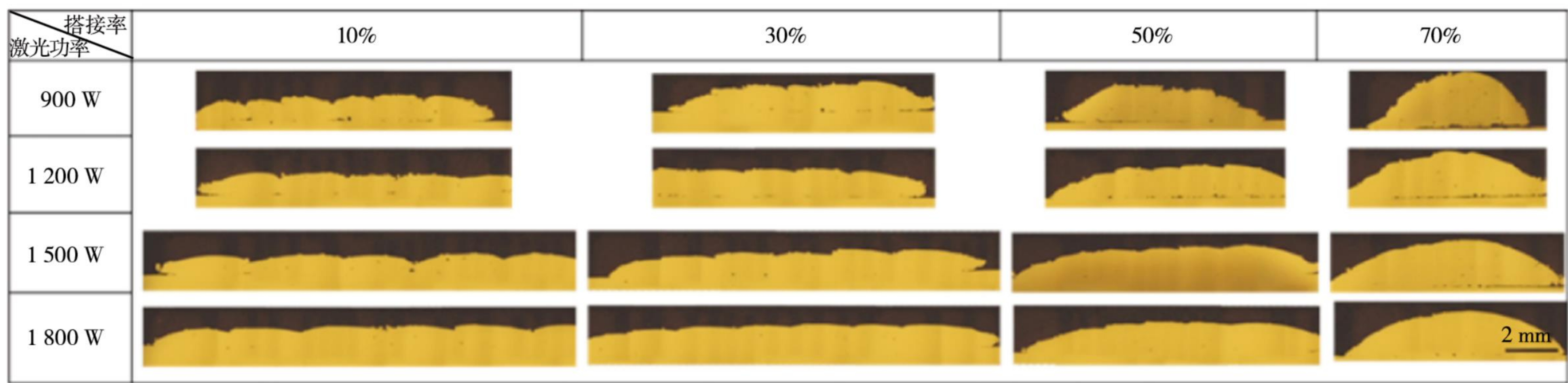
图7 不同搭接率与激光功率组合下LDED单层多道沉积截面形貌 Fig. 7 The cross-sectional morphologies of single-layer multi-pass LDED deposits under different lap joint rate and laser power combinations
