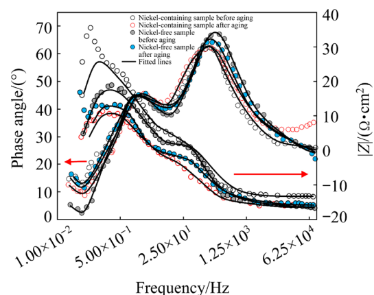
Fig. 9 Bode plots of nickel-containing and nickel-free samples
