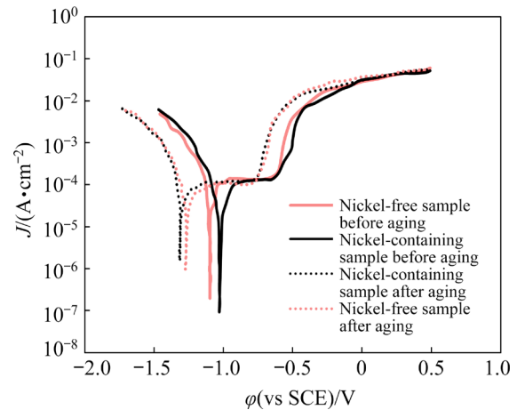
Fig. 7 Polarization curves of nickel-containing and nickel-free samples
