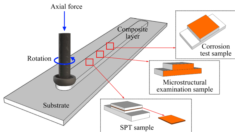
Fig. 1 Schematic illustration of extraction position of microstructural examination, SPT test, and corrosion examination samples (The highlighted area shows the position of the examination)
