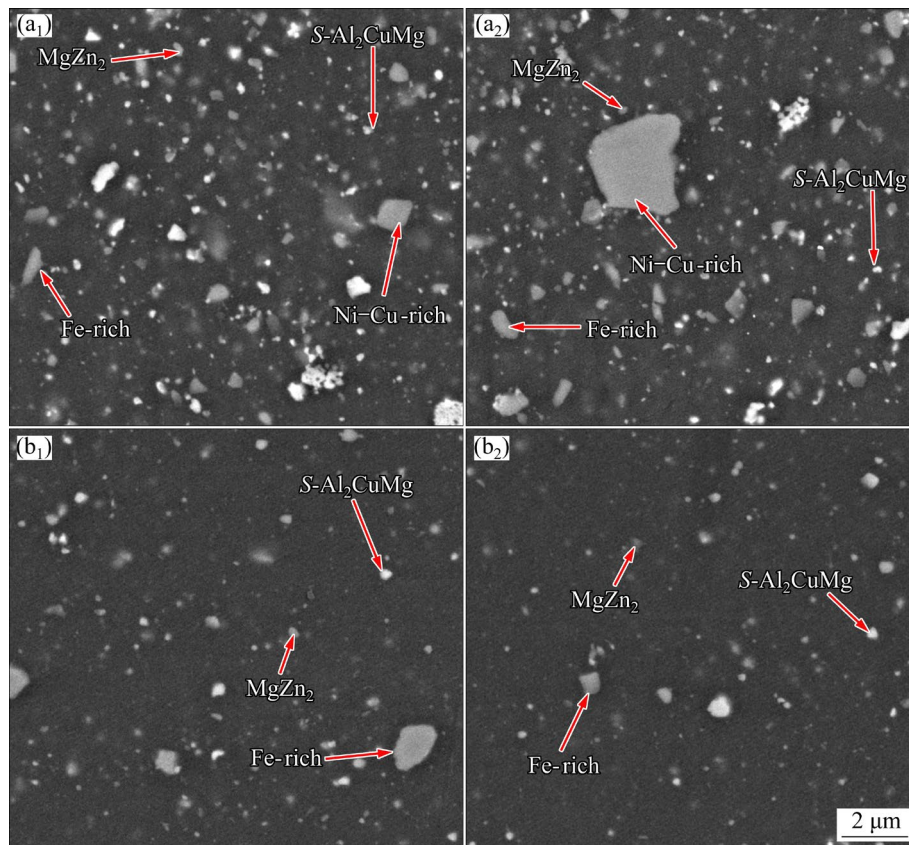
Fig. 5 SEM images of precipitates and second phase particles of samples before (a 1 , b 1 ) and after (a 2 , b 2 ) aging: (a 1 , a 2 ) Nickel-containing; (b 1 , b 2 ) Nickel-free
