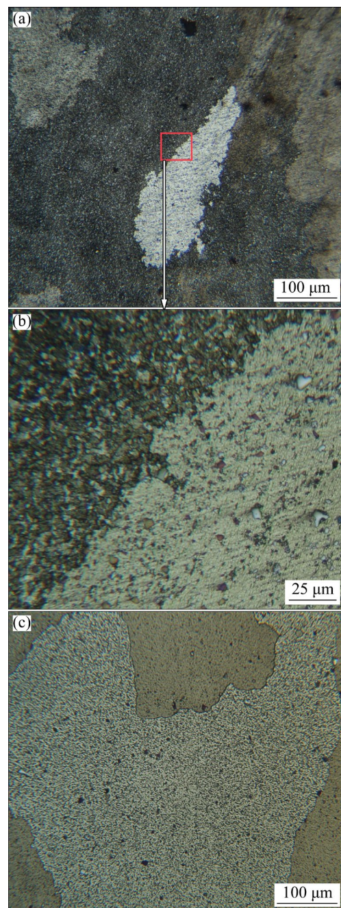
Fig. 4 Microstructure of center zone of samples after artificial aging heat treatment: (a, b) Nickel-containing; (c) Nickel-free
