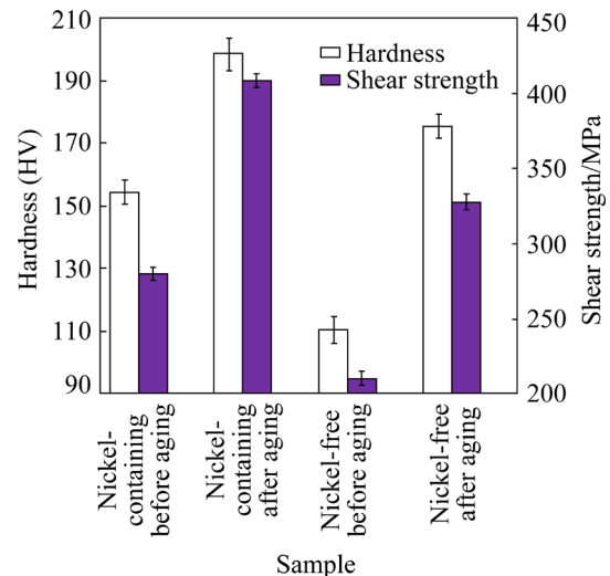
Fig. 6 Average hardness and shear strength of different samples
