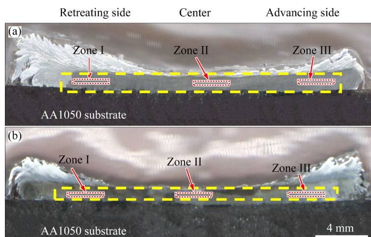
Fig. 2 Cross-section of samples: (a) Nickel-free; (b) Nickel-containing
