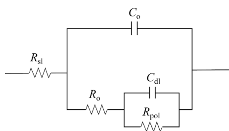
Fig. 10 Model used to investigate corrosion behavior
