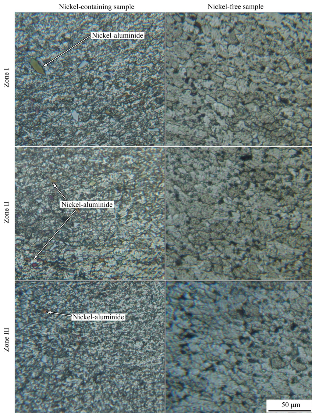
Fig. 3 Optical microscope images of different areas of nickel-containing and nickel-free samples
