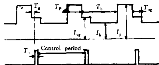
T_g - Time taking image, I_{vg} - Current taking image T_p - Peak time, I_p - Peak current, T_i - Imageing time T_b - Basic time, I_b - Basic current, T_d - Delay time
