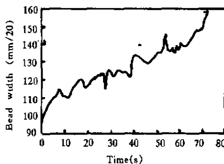
(a) Top - bead width of weld seam
