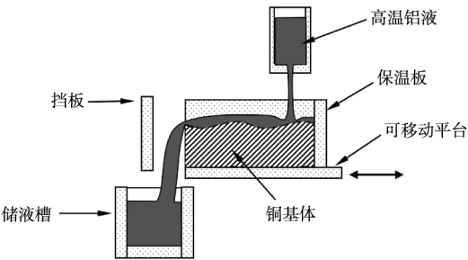
图1 冲击射流固-液复合法制备铜/铝复合材料示意图 Fig. 1 Schematic diagram of the preparation of copper/aluminum composites by impact jet solid-liquid compound method
