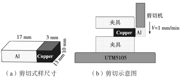
图2 剪切试样尺寸及剪切示意图 Fig. 2 Size of the shear sample and shear schematic diagram
